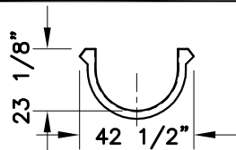
32" Open Flume
