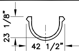
32" Open Flume
